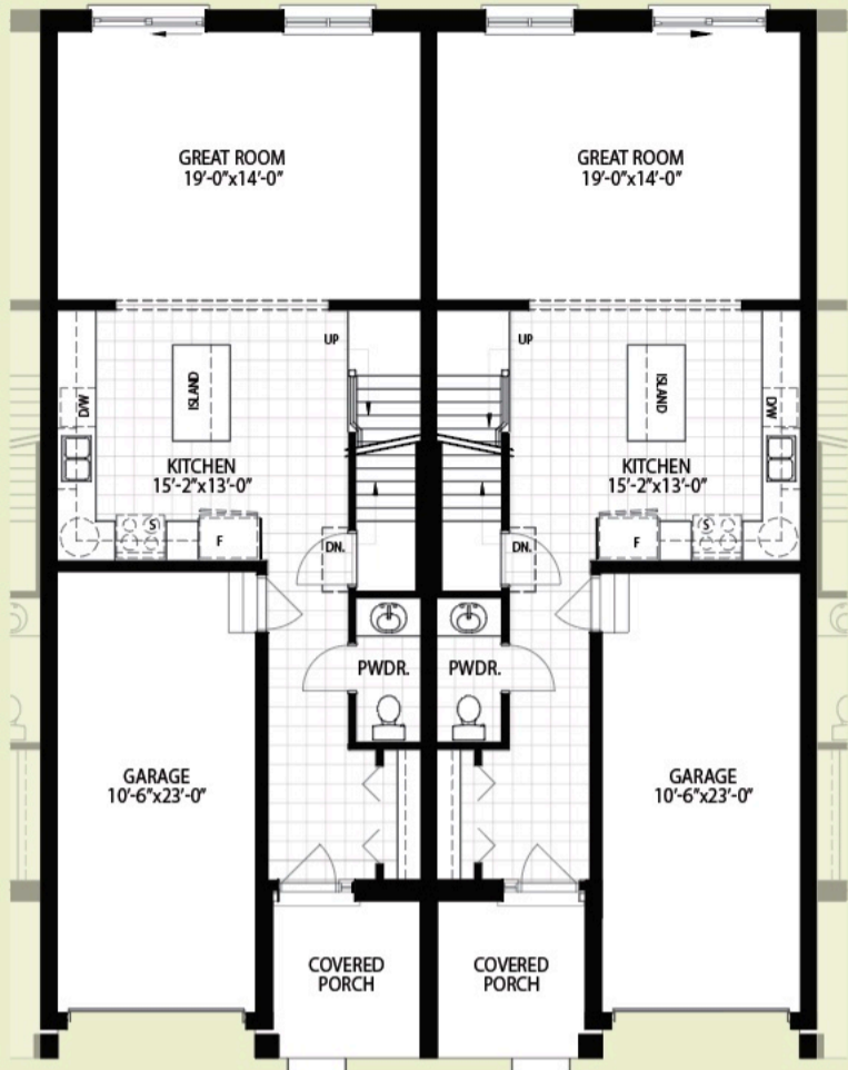
Main Floor Plan 725 sq.ft.
