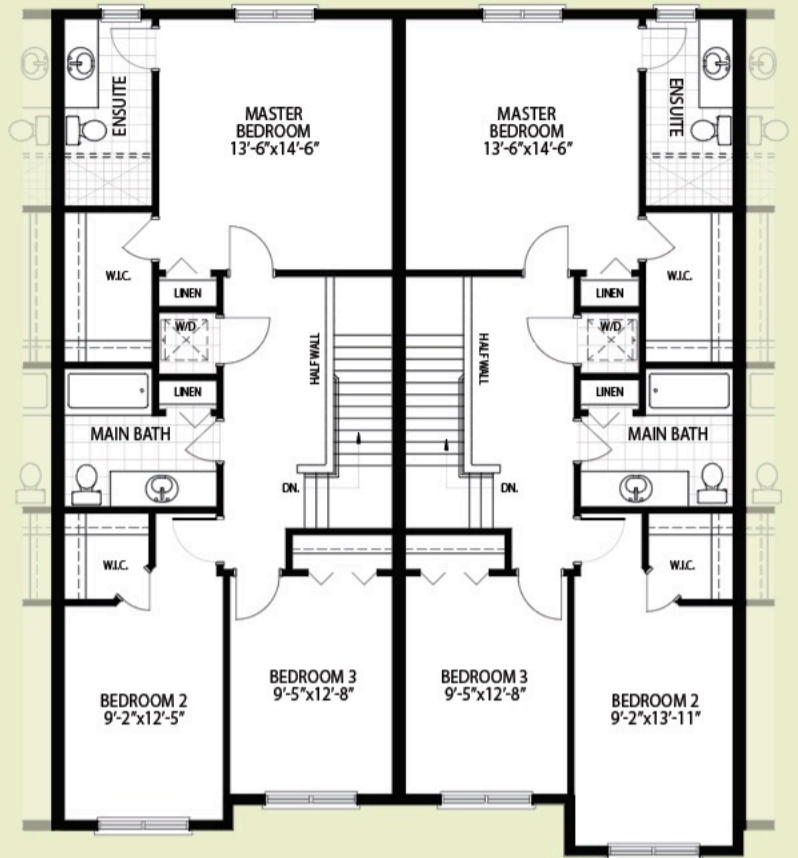
Second Floor Plan 925 sq.ft.
